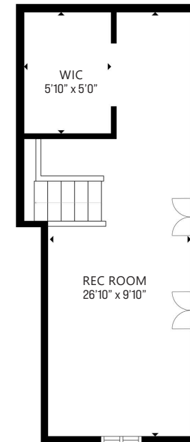
UPPER LEVEL: 255 SQ.FT.
