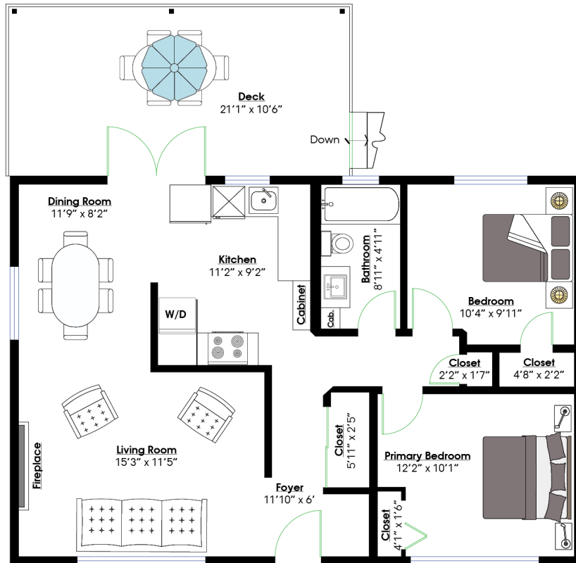
MAIN LEVEL Floor Area: 852 Sq. Ft. Ceiling Height: 8'
