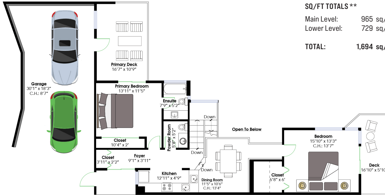
MAIN LEVEL Floor Area: 965 Sq. Ft. Ceiling Height: 8'
