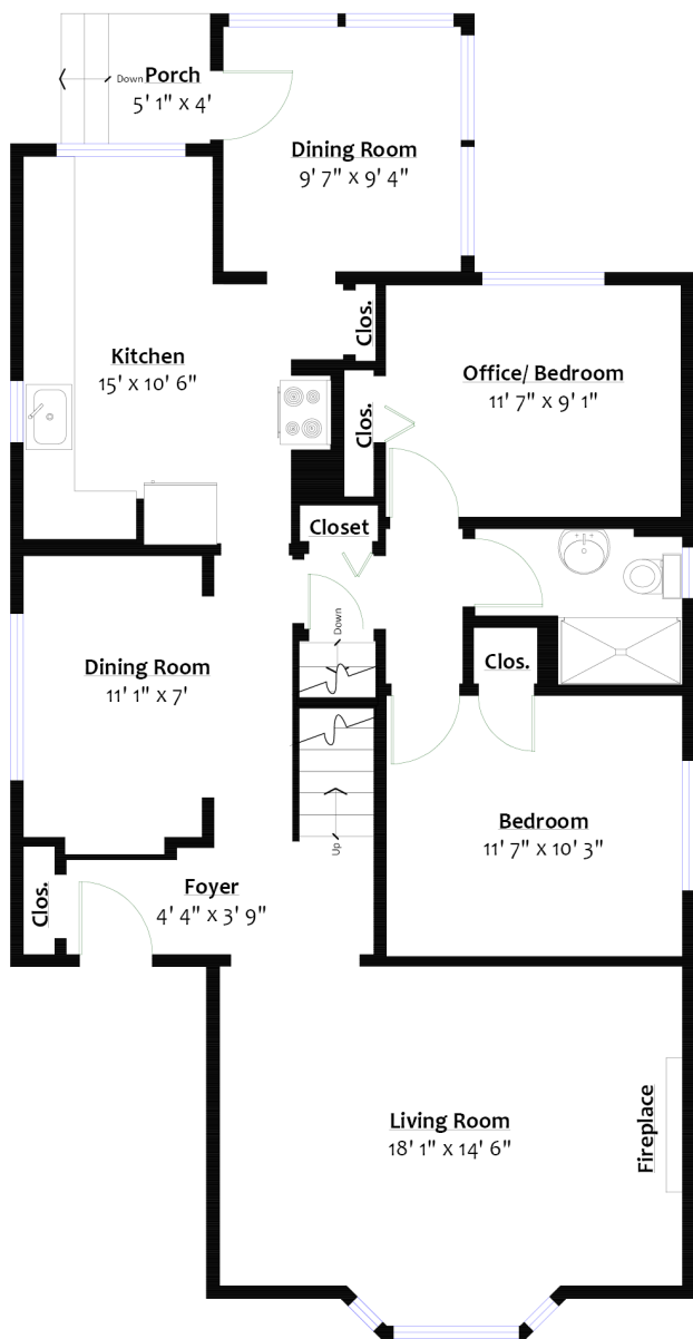
MAIN LEVEL Floor Area: 1,132 Sq. Ft. Ceiling Height: 8' 3"
