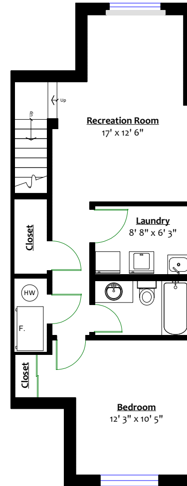
LOWER LEVEL Floor Area: 657 Sq. Ft.
