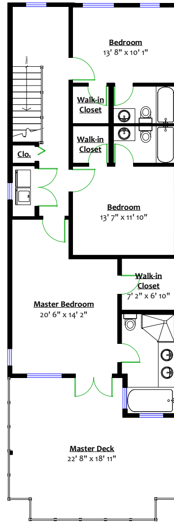
UPPER LEVEL Floor Area: 1,161 Sq. Ft.
