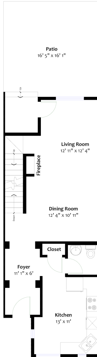
MAIN LEVEL Floor Area: 653 Sq. Ft.
