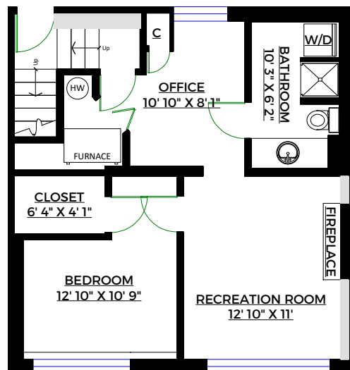
LOWER LEVEL Floor Area: 560 Sq. Ft.
