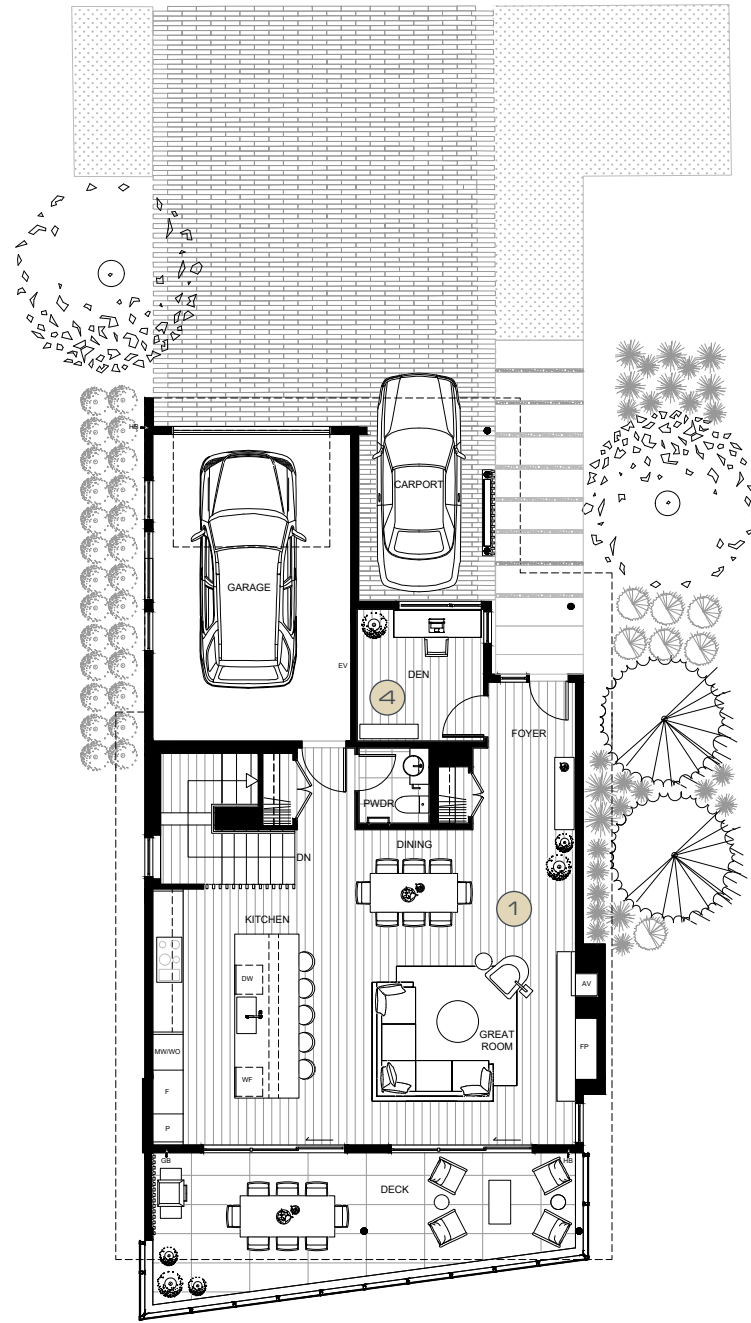
Main Level
